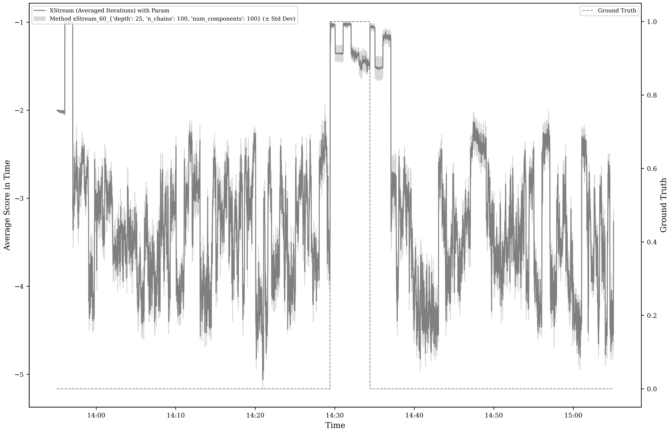
Method XStream Score for Scenario A2
